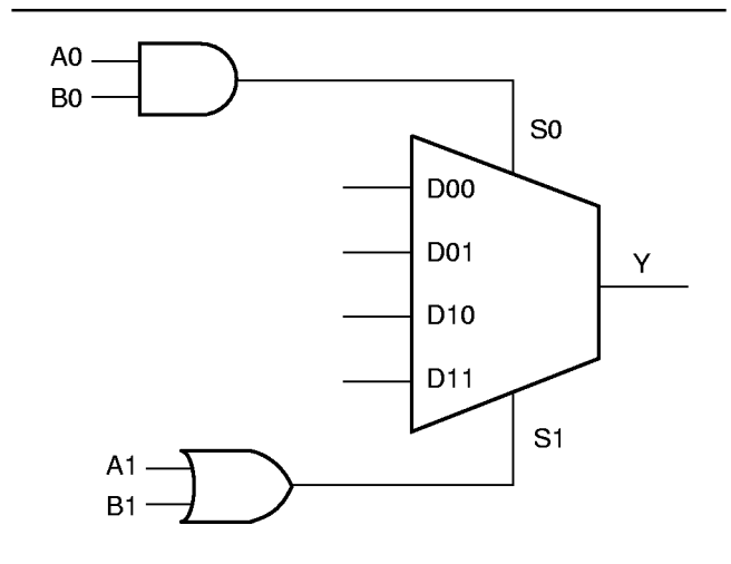
Figure 1 • C-Module Implementation
